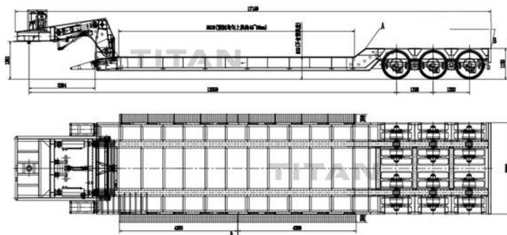
3 line 6 axle removable gooseneck lowboy trailer drawing
