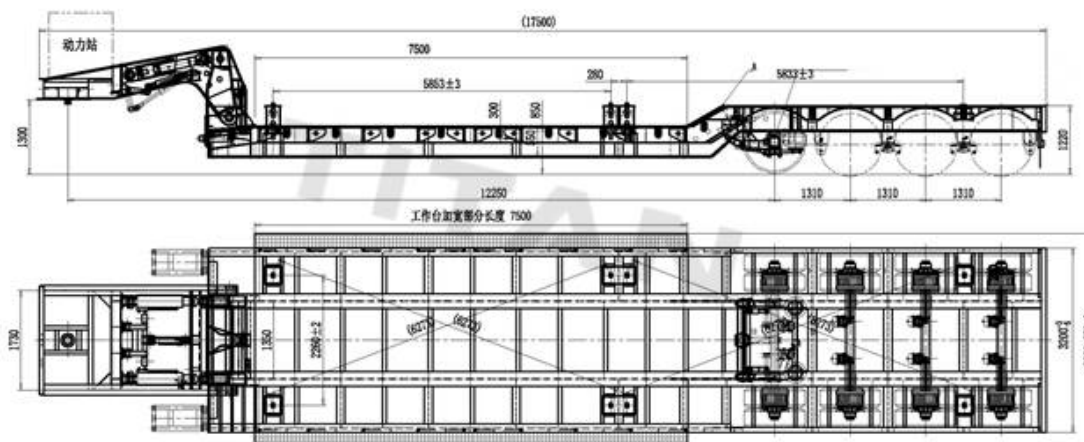
4 axle front loading lowbed trailer technical parameter drawing
