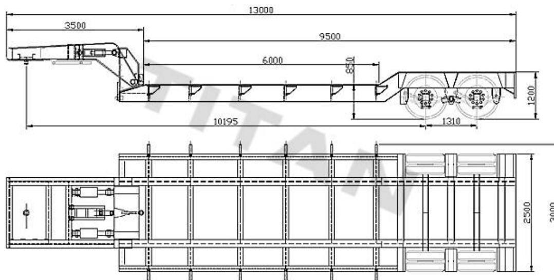
2 axle detachable gooseneck lowbody trailer drawing
