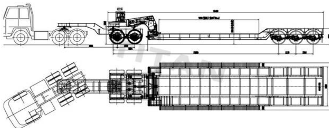
3 axle lowboy trailer with 2 axle dolly technical specification
