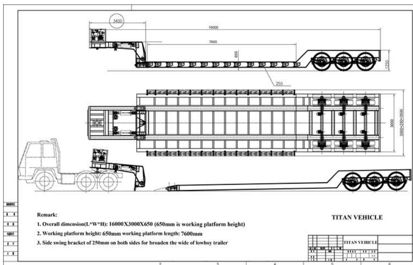
TITAN 3 axle detachable gooseneck lowboy trailer drawing
